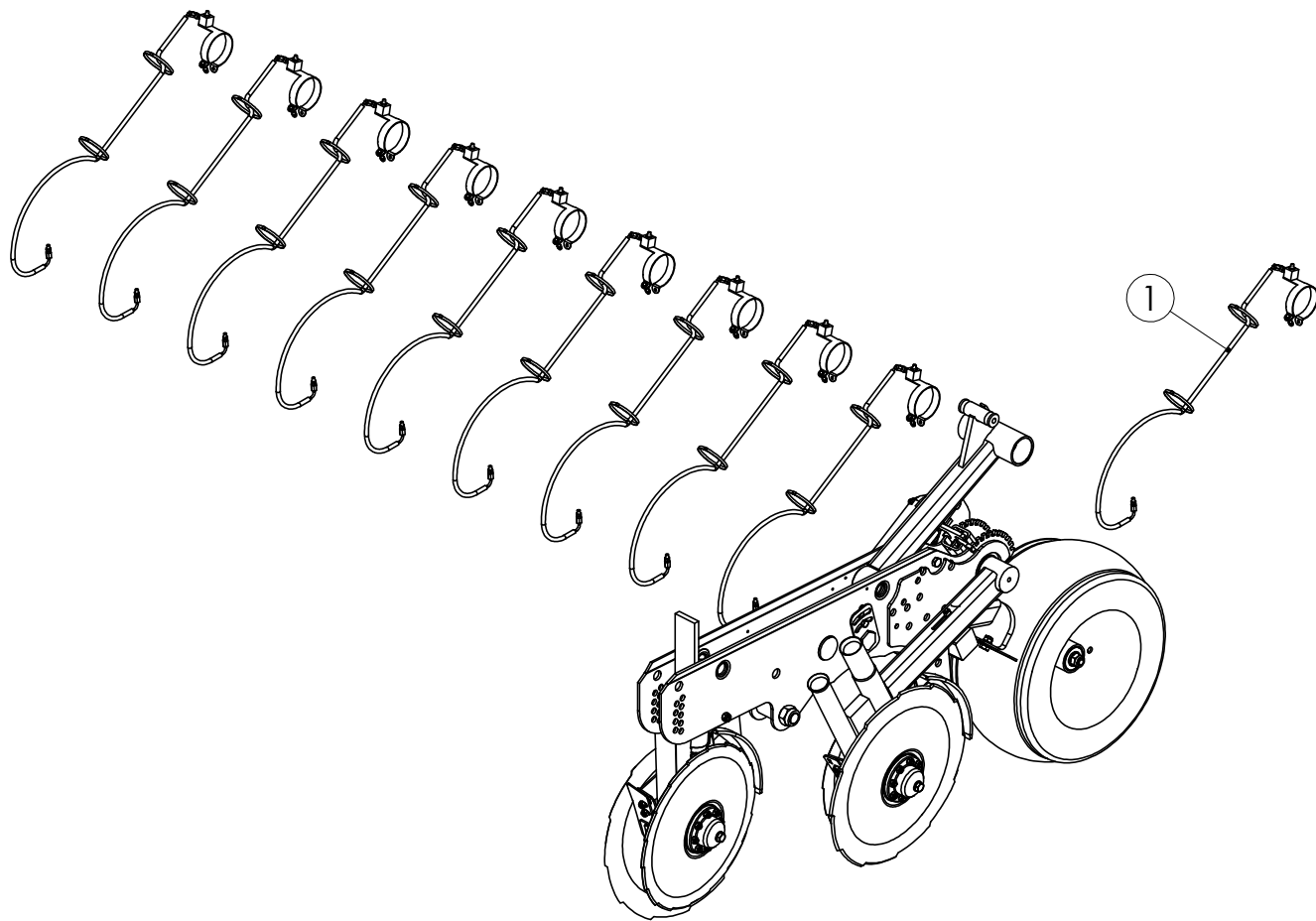
99218803 Grease nipple
